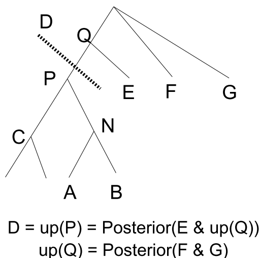
Figure 3. Traversing a tree with up-posteriors. FastTree optimizes the tree near node N by analyzing the posterior distributions for subtrees A, B, and C, as well as the “up-posterior” D.
